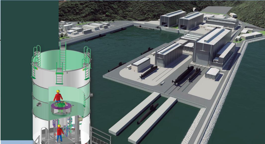
P roject of the new SETT (Submarine Escape Training Tank) and Flooding Simulator for submarines in the Shipyard and Naval Base of Itaguaí.
